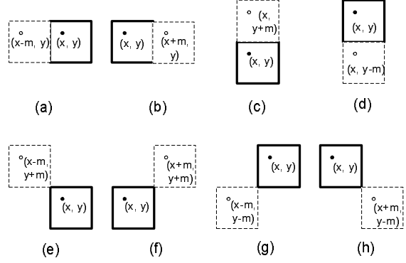
Figure 6. Virtual image construction process in 2-dimensional square input domain
