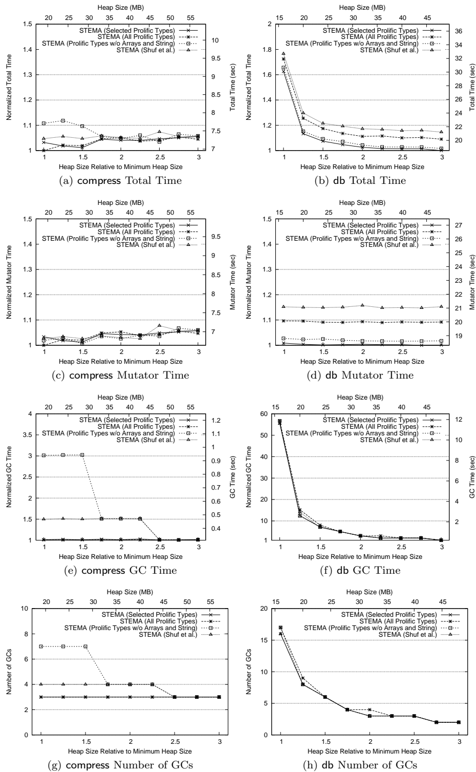
Fig. 26. Effects of Choice of Prolific Types on compress and db
