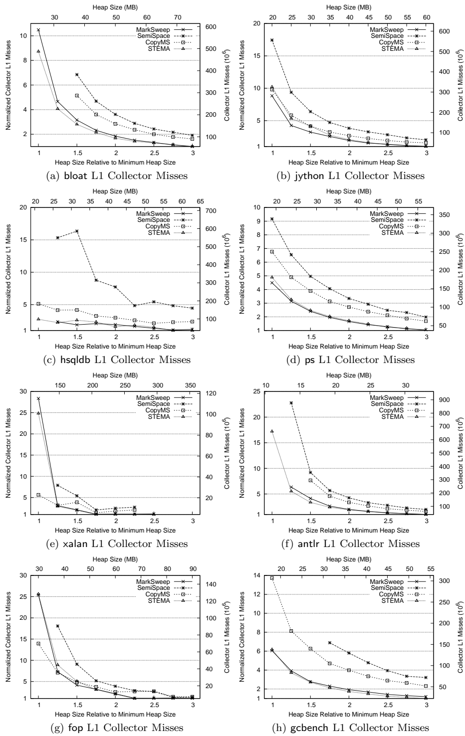
Fig. 21. STEMA vs. Other Collectors (Total L1 Collector Misses)
