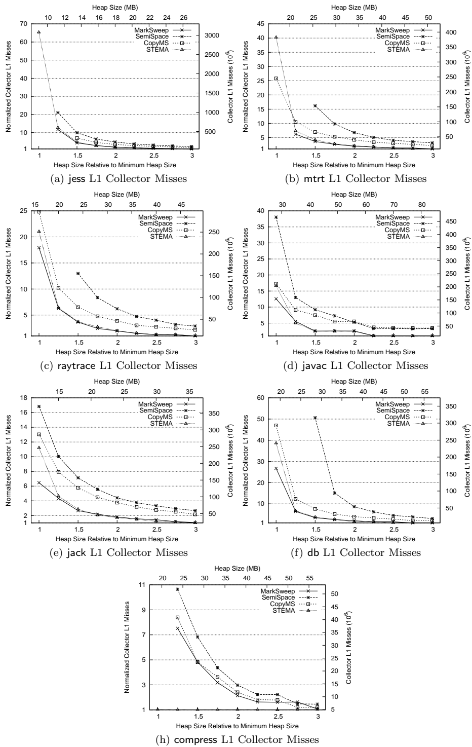
Fig. 20. STEMA vs. Other Collectors (Total L1 Collector Misses)
