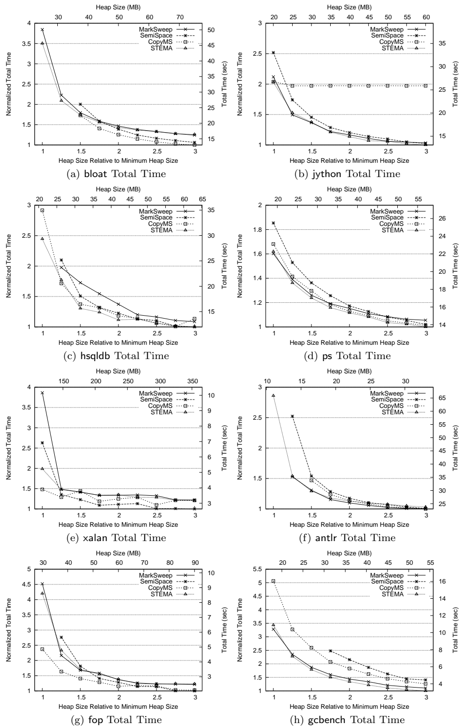
Fig. 13. STEMA vs. Other Collectors (Total Execution Time)
