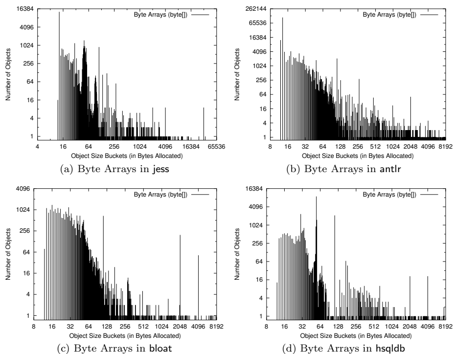
Fig. 7. Size Distribution of Byte Arrays
