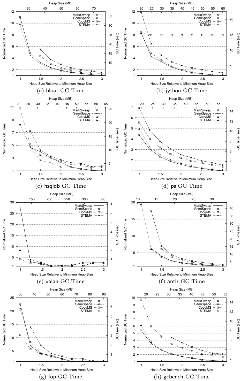
Fig. 17. STEMA vs. Other Collectors (Total GC Time)
