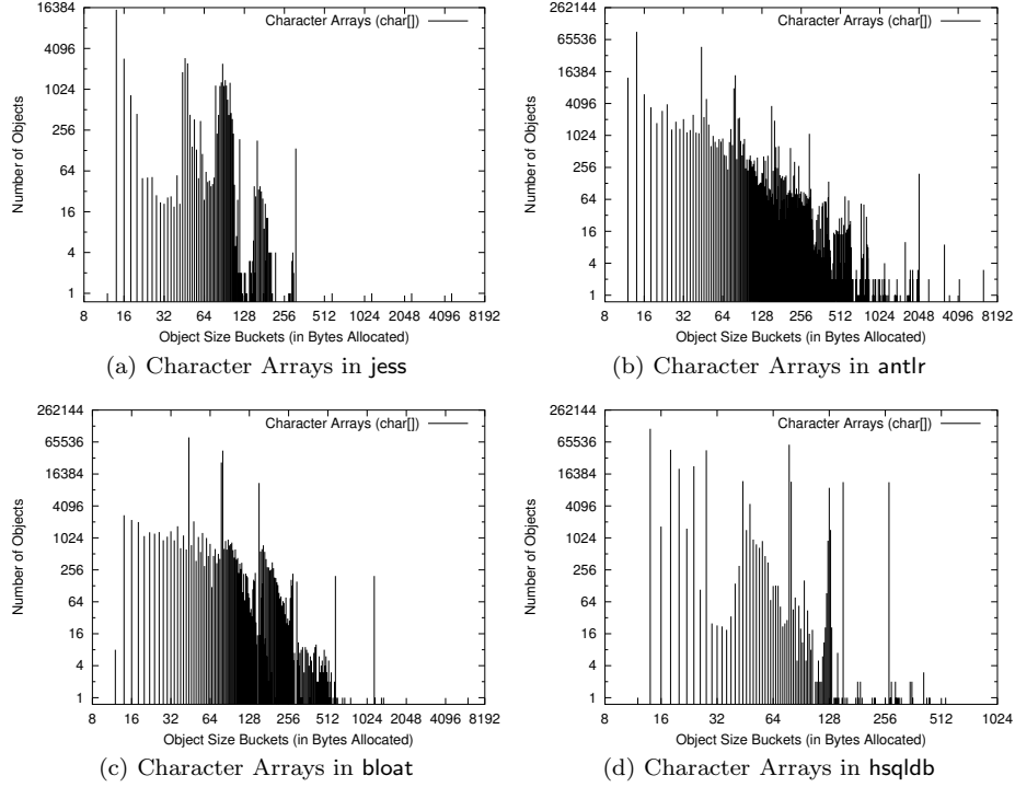
Fig. 8. Size Distribution of Character Arrays
