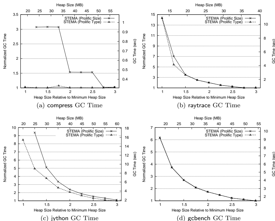
Fig. 29. Prolific Sizes vs. Prolific Types (Total GC Time)
