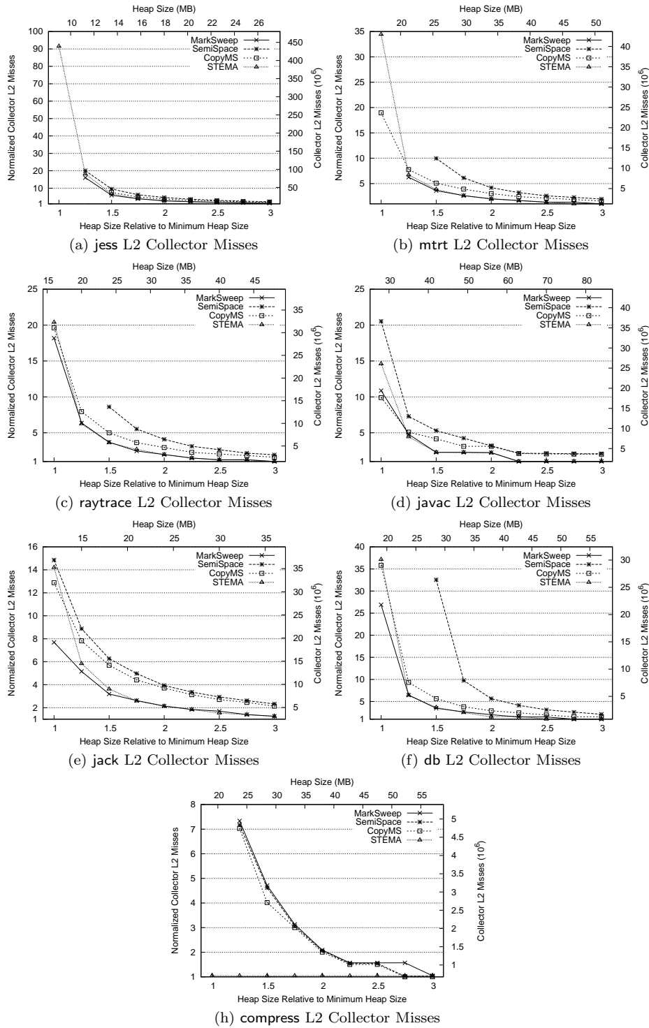
Fig. 24. STEMA vs. Other Collectors (Total L2 Collector Misses)
