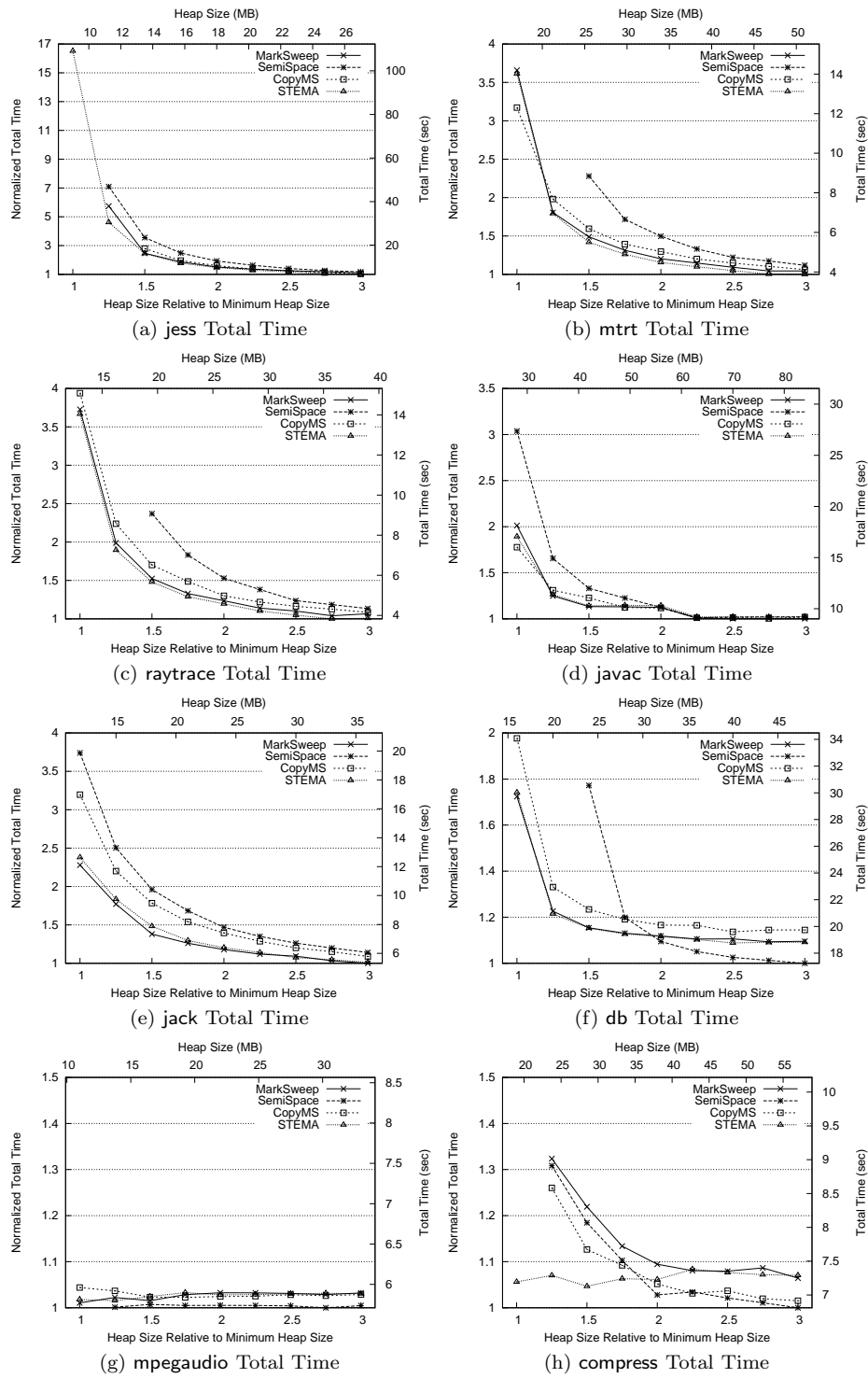
Fig. 12. STEMA vs. Other Collectors (Total Execution Time)
