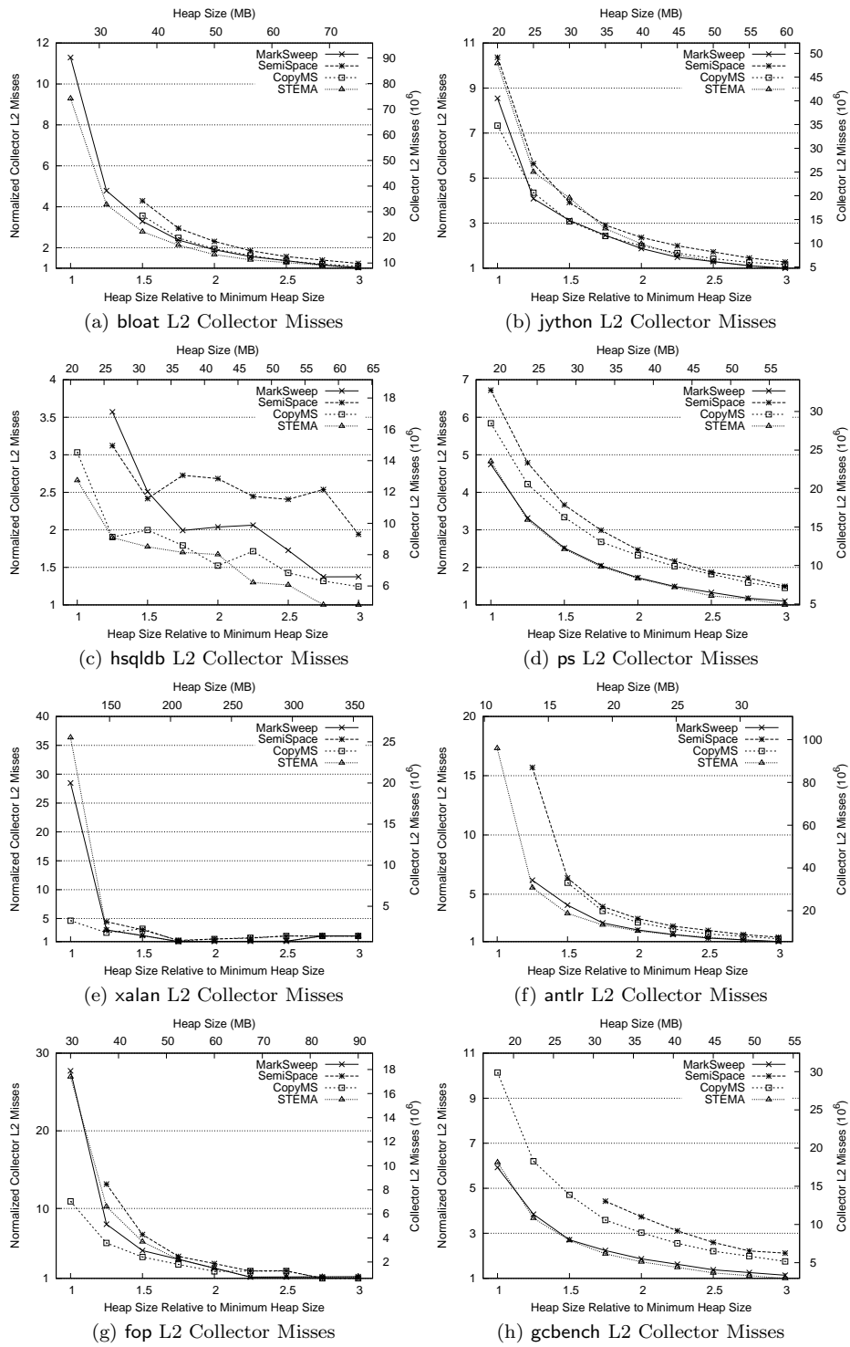
Fig. 25. STEMA vs. Other Collectors (Total L2 Collector Misses)
