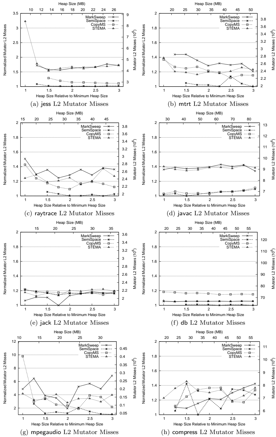
Fig. 22. STEMA vs. Other Collectors (Total L2 Mutator Misses)
