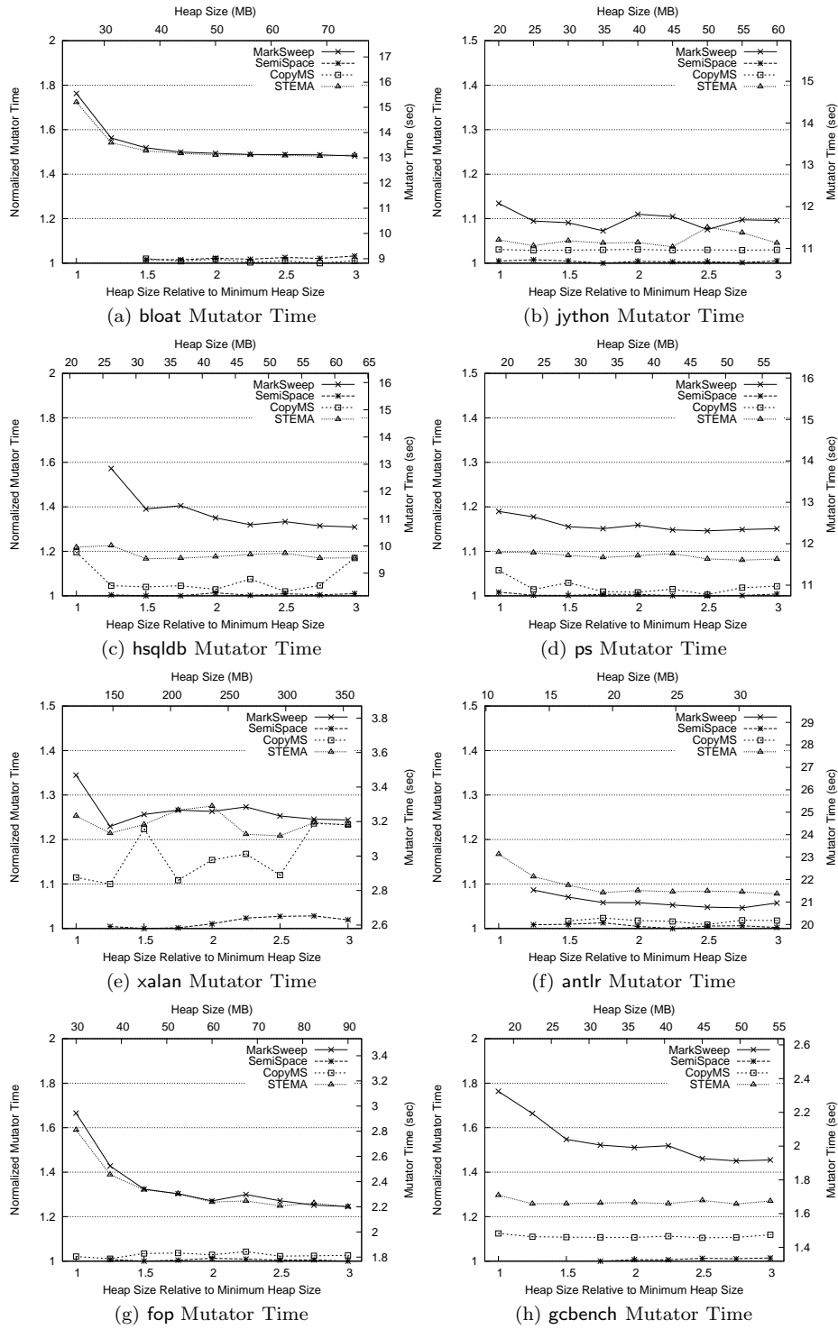
Fig. 15. STEMA vs. Other Collectors (Total Mutator Time)
