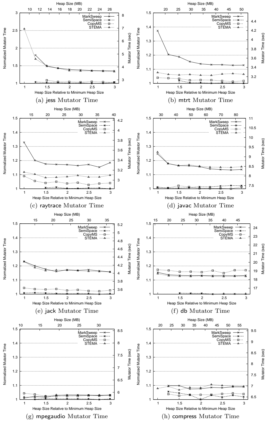
Fig. 14. STEMA vs. Other Collectors (Total Mutator Time)
