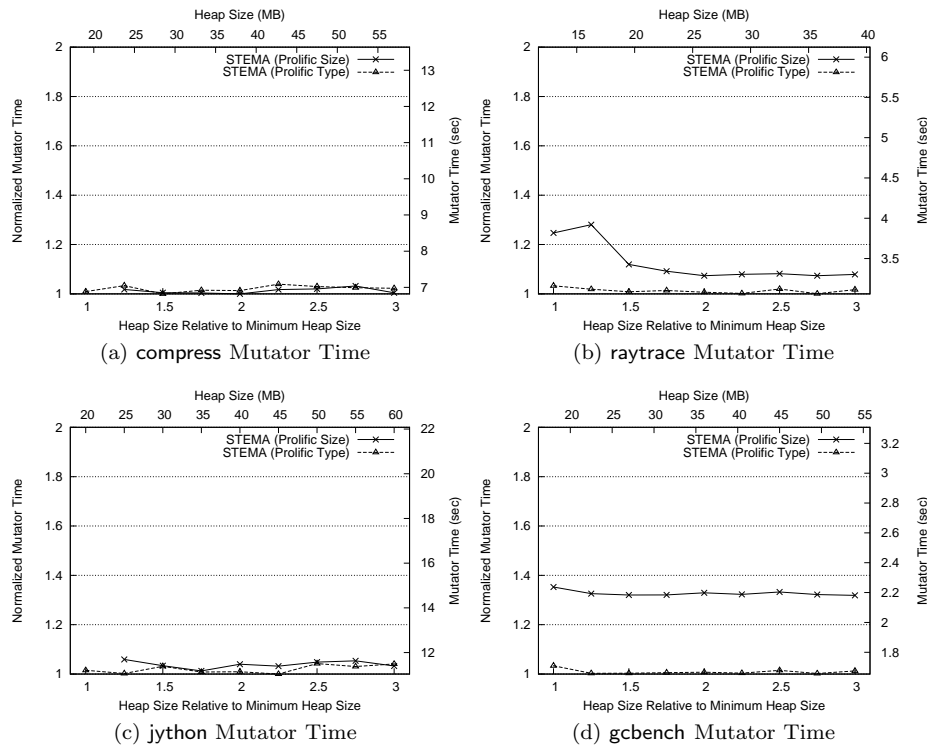
Fig. 28. Prolific Sizes vs. Prolific Types (Total Mutator Time)
