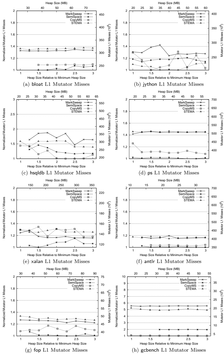
Fig. 19. STEMA vs. Other Collectors (Total L1 Mutator Misses)
