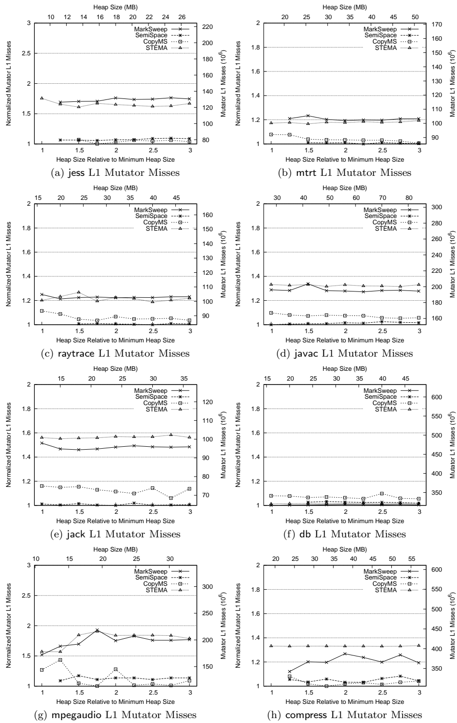
Fig. 18. STEMA vs. Other Collectors (Total L1 Mutator Misses)
