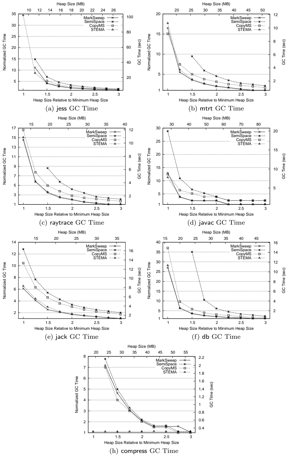
Fig. 16. STEMA vs. Other Collectors (Total GC Time)
