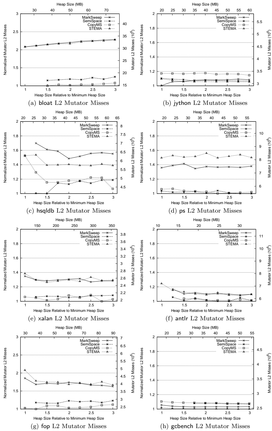
Fig. 23. STEMA vs. Other Collectors (Total L2 Mutator Misses)
