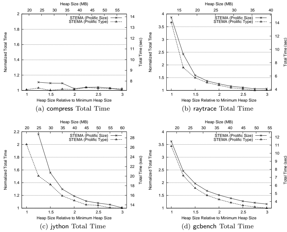
Fig. 27. Prolific Sizes vs. Prolific Types (Total Execution Time)
