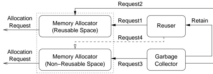
Fig. 9. STEMA: Reuser, Memory Allocators, and Garbage Collector
