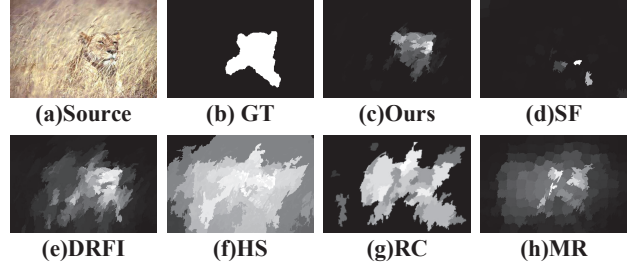
Fig. 1: An example illustrating that saliency models based on handcrafted low-level features are fragile. From top left to bottom right: source image, ground truth, our saliency map, and saliency maps of other five latest methods, including SF[13], DRFI[14], HS[15], RC[16], and MR[17].
