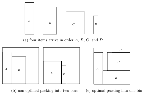
Figure 1: Example of optimal packing and non-optimal packing
