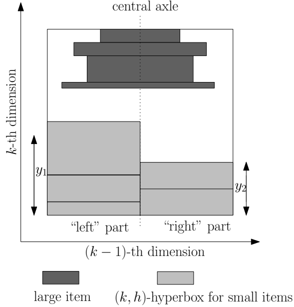
Figure 2: Packing k -dimensional items into k -dimensional hypercube.
