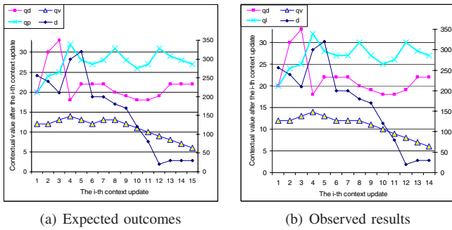
Fig. 3. Spot the difference: Challenge of obscured failures in integration testing of ubiquitous computing applications.
