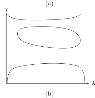
Figure 3: Two ellipsoids moving under quartic rational motions.
