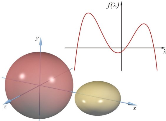
Figure 1: Two ellipsoids and their characteristic polynomial f(\lambda) .
