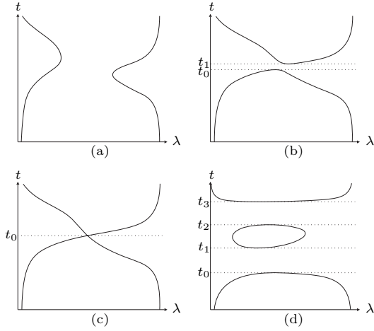
Figure 2: Typical topologies of the zero sets for two moving ellipsoids that are (a) separate because there are two distinct negative roots for all t ; (b) overlapping when t \in [t_0, t_1] indicated by the absence of negative roots; (c) separate until t = t_0 when they touch each other and then separate again; (d) overlapping when t \in [t_0, t_1] and [t_2, t_3] .
