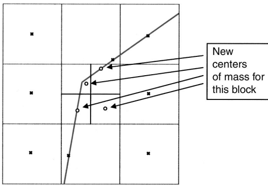
Fig. 7 Dividing the central block into four rectangular subblocks.
