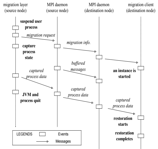
Fig. 2. Process migration steps in M-JavaMPI
