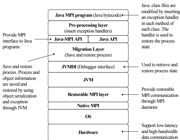
Fig. 1. The layered design of M-JavaMPI
