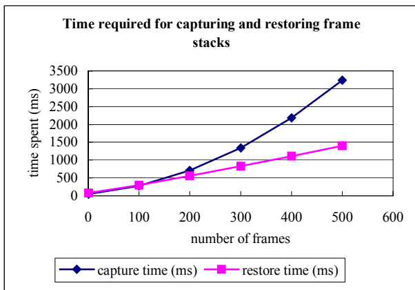
Fig.6. Time spent in capturing and restoring frames
