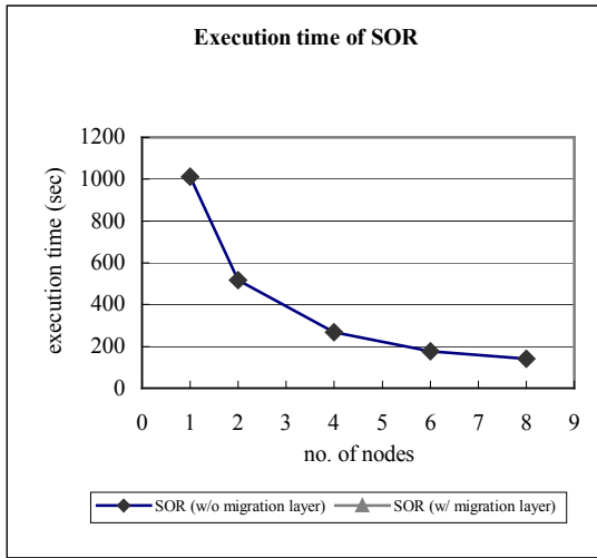
Fig. 8. Time spent in executing SOR using different numbers of nodes with and without migration layer
